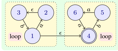
Figure 2: A \langle 3, 2 \rangle -flat automaton of (ab)^* \bullet (baa)^* .
