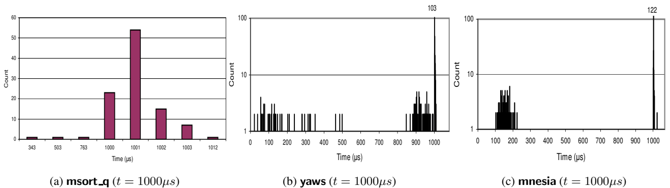
Figure 4: Counts of pause times (in \mu s ) for the time-based incremental collector.
