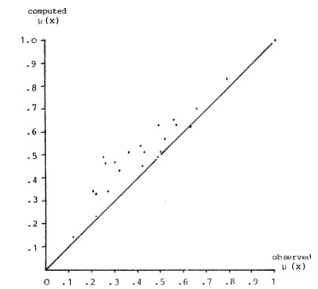
Fig. 6. Arithmetic mean: Observed versus computed grades of membership.
