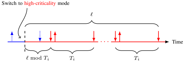
Fig. 3. After fitting a number of full jobs into an interval of length \ell , there are \ell \bmod T_i time units left for either another full job, a carry-over job, or no job at all. In this figure it is enough for a carry-over job.
