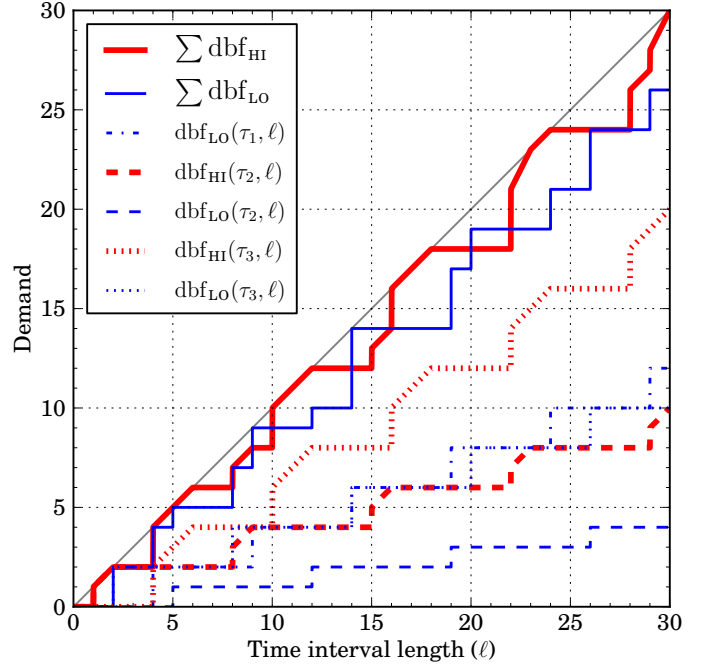
Fig. 7. Demand-bound functions for the tasks from Example II.1 after having low-criticality relative deadlines tuned by the algorithm in Fig. 5.
