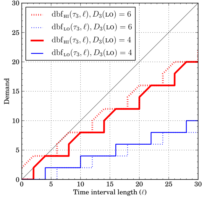
Fig. 4. Demand-bound functions for task \tau_3 from Example II.1 with two different values for D_3(\text{LO}) .
