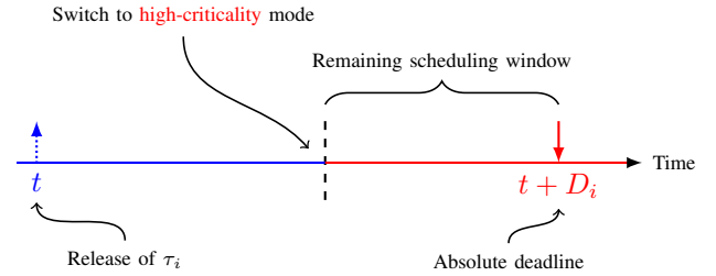
Fig. 1. After a switch to high-criticality mode, the remaining execution demand of a carry-over job must be finished in its remaining scheduling window.
