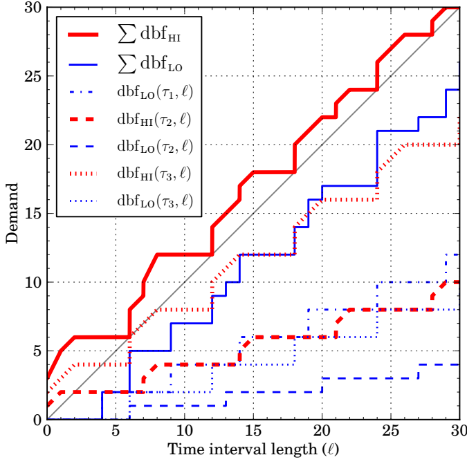
Fig. 6. Demand-bound functions for the tasks from Example II.1 with unmodified low-criticality relative deadlines ( D_i(\text{LO}) = D_i(\text{HI}) = D_i ).
