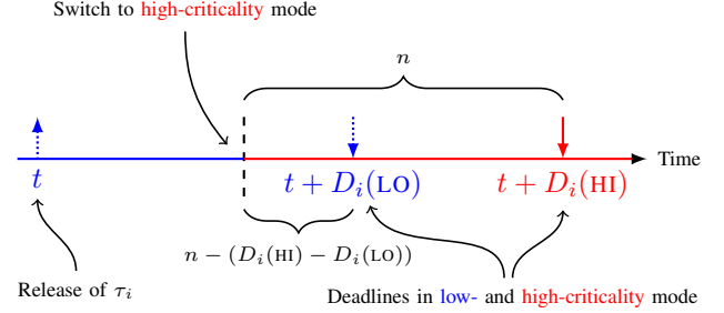
Fig. 2. A carry-over job of \tau_i has a remaining scheduling window of length n after the switch to high-criticality mode. Here the switch happens before the job’s low-criticality deadline.
