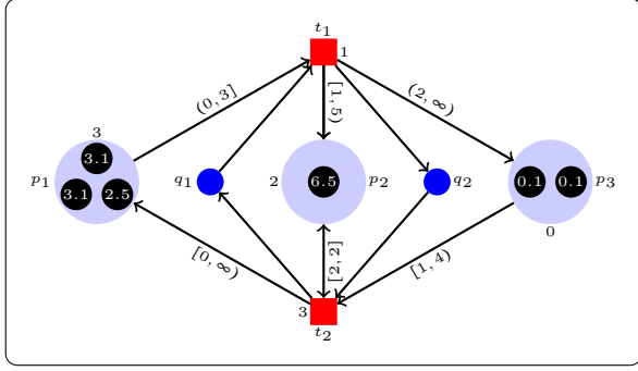
Fig. 1. A simple example of a PTPN.
