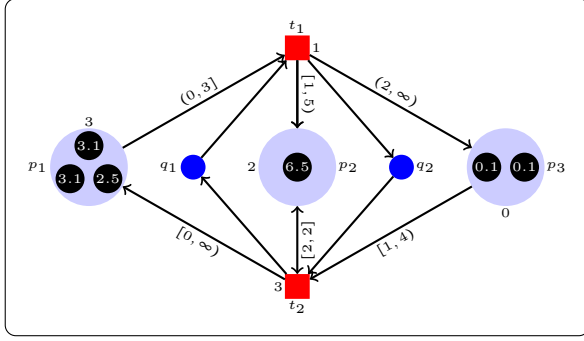
Fig. 1. A simple example of a PTPN.
