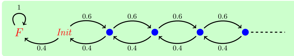
Fig. 4. A Markov chain that is not decisive.
