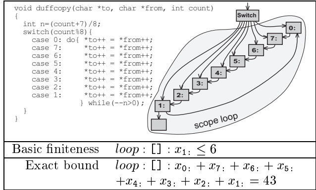
Figure 15. Multiple-entry loop: duff
