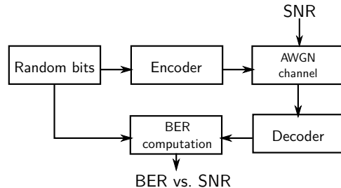
Figure 2: Block diagram of the simulation framework. In each run of the simulation, we encode a large number of random bits, transform the resulting chip sequences with an AWGN channel, and then decode them again.
