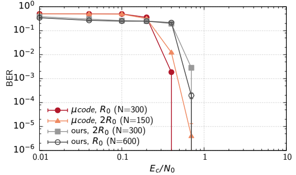
Figure 5: Comparison of BER vs E_c/N_0 between \mu code and our new approach for different numbers of chips per symbol. Our results suggest that even though our approach increases the data rate, a better performance gain is obtained by reducing the number of chips per symbol when conditions allow.
