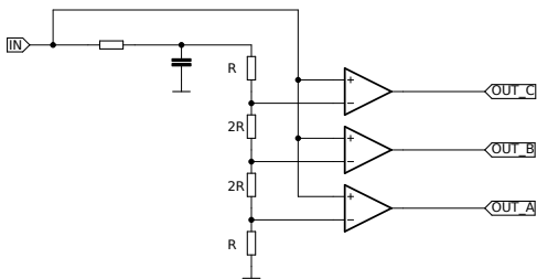
Figure 7: Thresholding circuit for a 2-bit per symbol code. The proposed thresholding stage uses three comparators rather than one to decode two-bits-per-symbol codes while remaining backwards-compatible to single-bit encoding.
