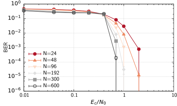
Figure 4: BER vs E_c/N_0 for different number of chips per symbol ( N ) in our approach. As expected, increasing the number of chips per symbol increases robustness at the cost of data rate.
