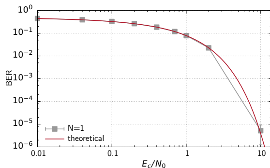
Figure 3: Comparison of the theoretical BER curve of PCM to our equivalent simulated results. Our simulation generates an almost perfect match to the theoretical values.
