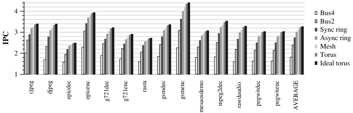
Figure 8: Comparing 8-cluster topologies
