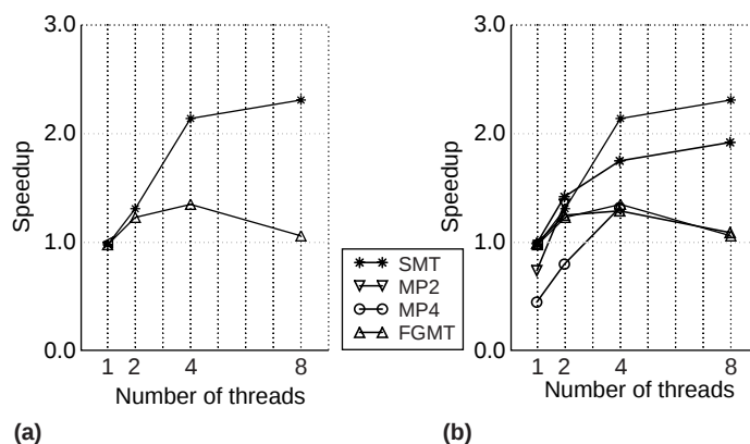
Figure 2. Speedups with the multiprogramming workload (a) and parallel workload (b).
