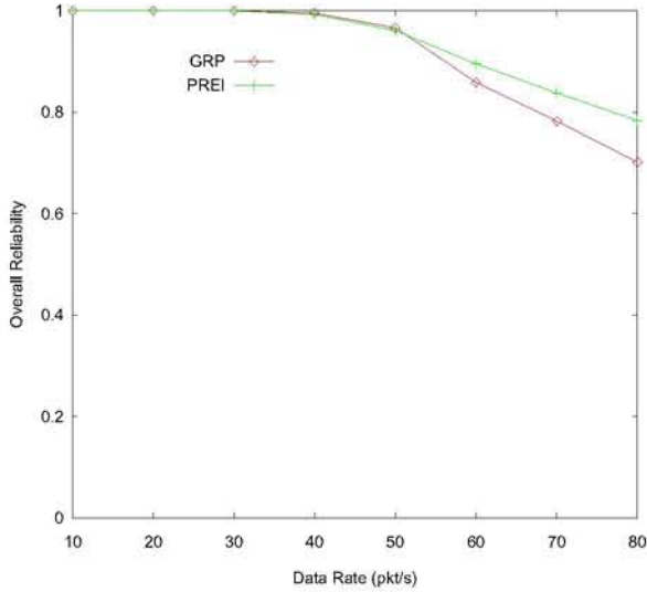
Fig. 6. Overall Reliability.
