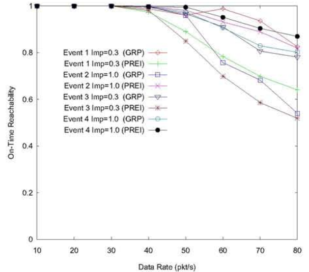
Fig. 4. On-Time Reachability.
