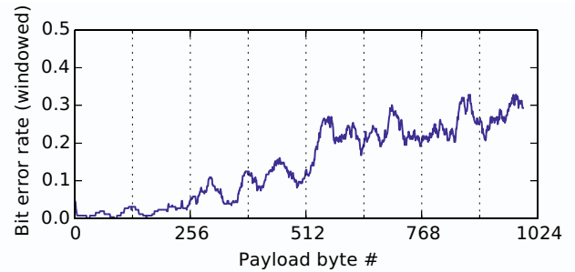
Fig. 2: A receiver's bit error rate over increasing byte positions, which correspond to increasing frequencies by design of the proposed scheme. Thus the plot shows that higher frequencies coincide with higher error rates.
