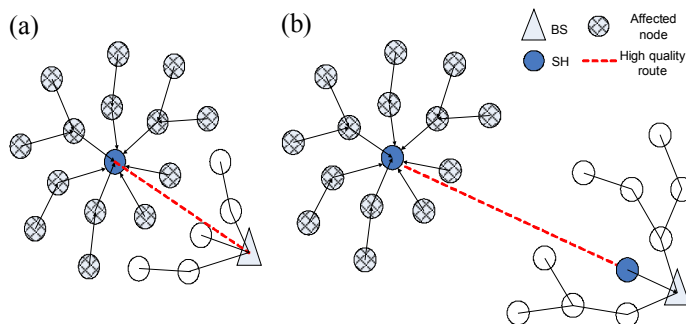
Fig. 1. Two examples of sinkhole attack in wireless sensor networks. (a) Using an artificial high quality route; (b) Using a wormhole.
