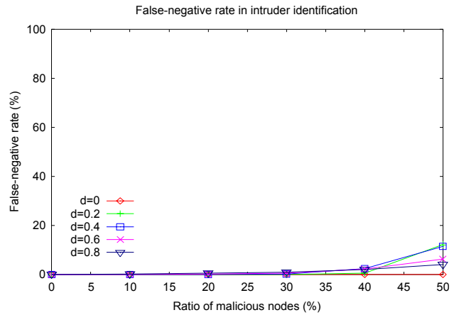
Fig. 8. False-negative rate in intruder identification
