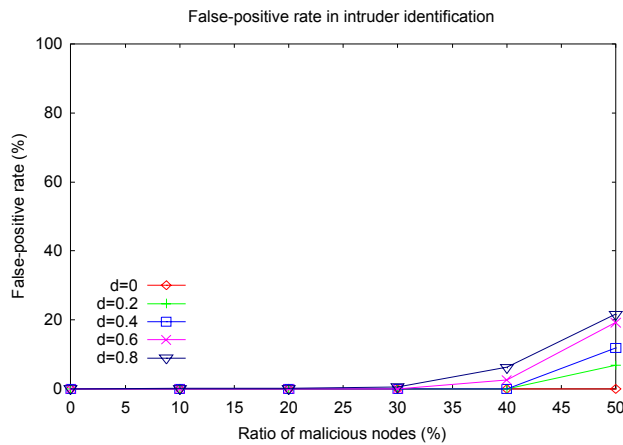
Fig. 7. False-positive rate in intruder identification
