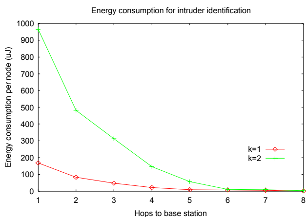
Fig. 10. Energy consumption for intruder identification
