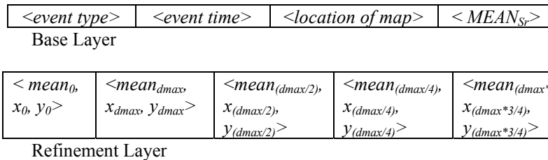
Figure 4 - Base Layer and Refinement Layer
