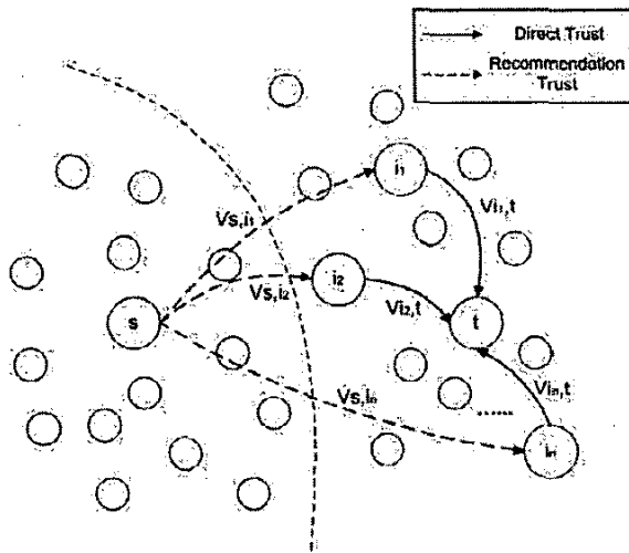
Figure 6. Trust Value Update
