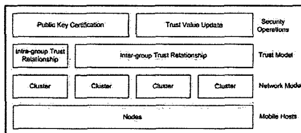
Figure 1. Architecture of Our Authentication Service
