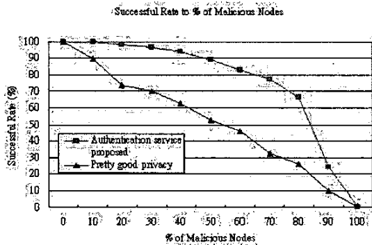
Figure 12. Comparison of Successful Rate to % of Malicious Nodes
