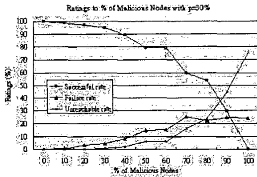
Figure 8. Ratings to % of Malicious Nodes with p=30\%
