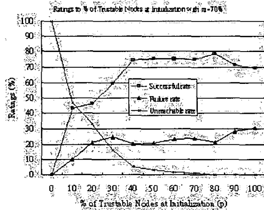
Figure 11. Ratings to % of Trustable Nodes with m=70\%
