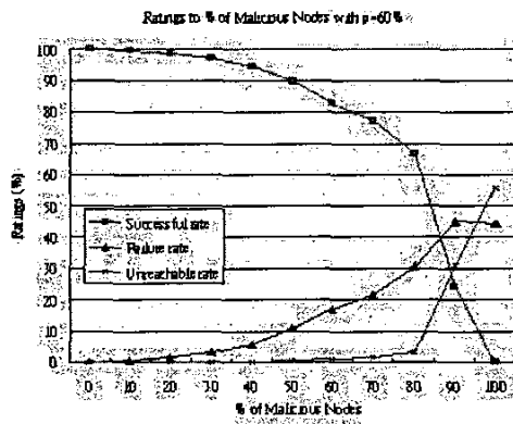
Figure 9. Ratings to % of Malicious Nodes with p=60\%
