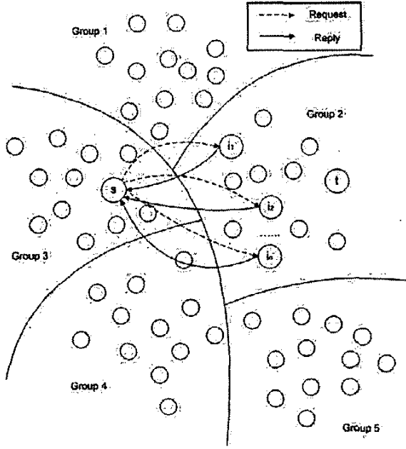
Figure 5. Public Key Certification
