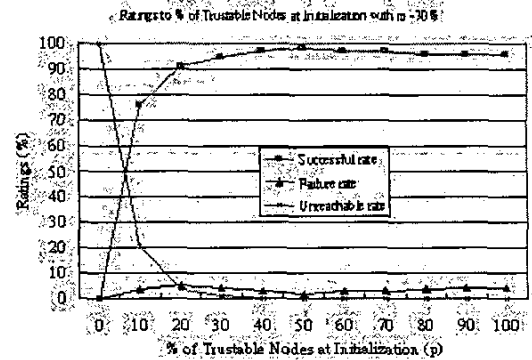
Figure 10. Ratings to % of Trustable Nodes with m=30\%
