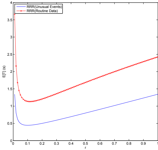
Fig. 4. After unusual events occur, travel delay with f=0.1 , D=10 , m=0.1 , \mu=100\text{pkt/s} , \tau=10\text{pkt/s} .
