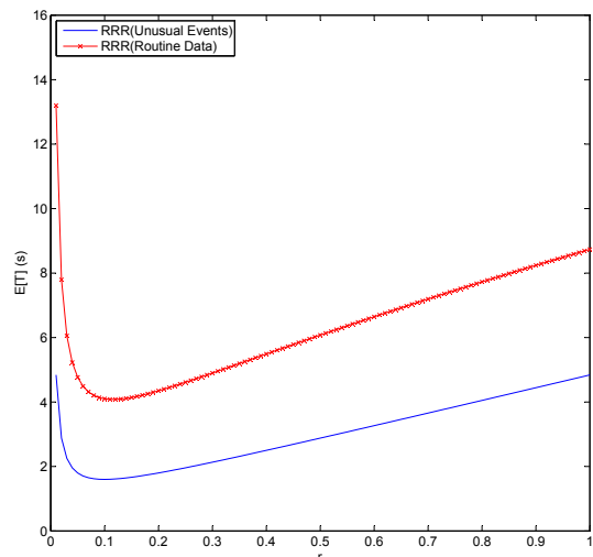
Fig. 2. After unusual events occur, travel delay with f=0.1 , D=10 , m=0.1 , \mu=30\text{pkt/s} , \tau=5\text{pkt/s} .
