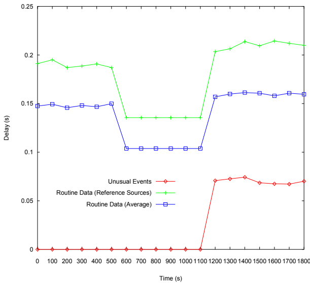
Fig. 7. Travel delay in three phases with f=0 , \lambda_U=5\text{pkt/s} , \lambda_R=1\text{pkt/s} , reference routine data sources at (30, 30), (30, 170), (170, 30), (170, 170).
