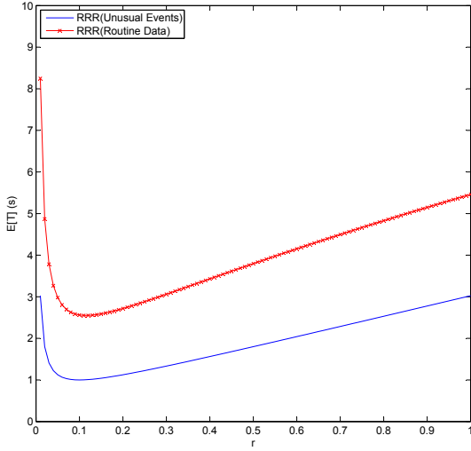
Fig. 3. After unusual events occur, travel delay with f=0.1 , D=10 , m=0.1 , \mu=50\text{pkt/s} , \tau=10\text{pkt/s} .
