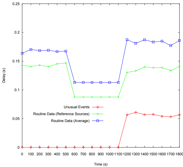
Fig. 6. Travel delay in three phases with f=0 , \lambda_U=5\text{pkt/s} , \lambda_R=1\text{pkt/s} , reference routine data sources at (30, 100), (170, 100), (100, 30), and (100, 170).
