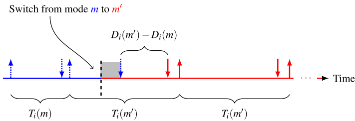
Fig. 8 The carry-over job is unaffected by the fact that the period of \tau_i was changed at the switch from m to m' . The minimum (remaining) scheduling window of a carry-over job is still the difference between the relative deadlines in the new and old mode, just as before with the standard model. As before, the remaining execution time budget for the job in the old mode m can be no larger the length of the interval between switch and deadline in m (the shaded interval)
