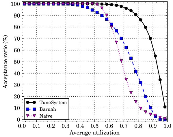
Fig. 14 P_{HI} = 0.5, R_T = 0.25, C^{\max} = 10 and T^{\max} = 200
