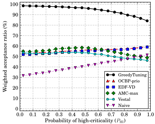
Fig. 11 P_{HI} varying, R_C = 4 , C_{LO}^{max} = 10 , T^{max} = 200 and R_D = 1
