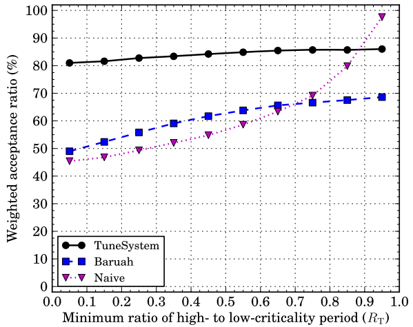
Fig. 15 P_{HI} = 0.5, R_T varying, C^{\max} = 10 and T^{\max} = 200
