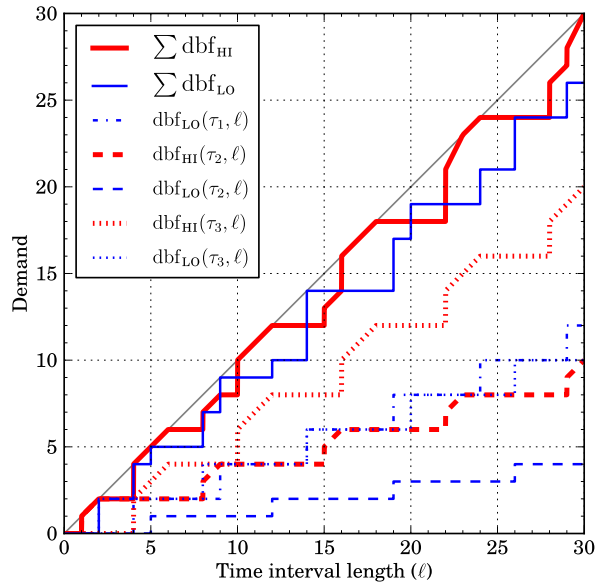
Fig. 6 Demand bound functions for the tasks from Example 1 after having low-criticality relative deadlines tuned by Algorithm 1
