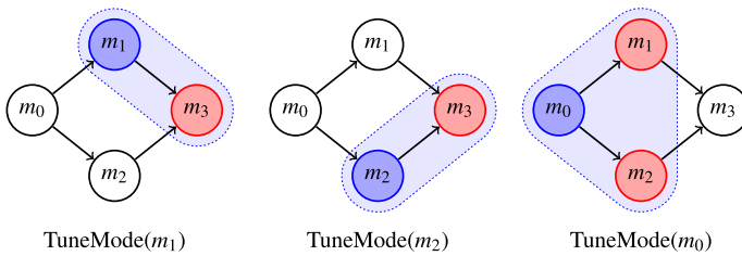
Fig. 9 The order in which modes are tuned by \text{TuneSystem}(\tau, G) , excluding the trivial \text{TuneMode}(m_3)
