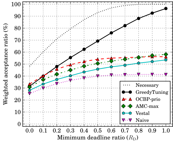
Fig. 13 P_{HI} = 0.5 , R_C = 4 , C_{LO}^{max} = 10 , T^{max} = 200 and R_D varying
