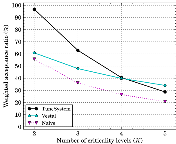
Fig. 17 R_C = 2 , C_{m_1}^{\max} = 10 , T^{\max} = 200 and K varying
