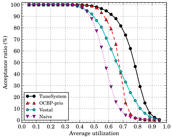
Fig. 16 R_C = 2, C_{m_1}^{\max} = 10, T^{\max} = 200 and K = 3
