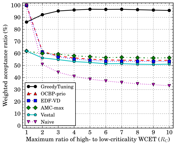
Fig. 12 P_{HI} = 0.5 , R_C varying, C_{LO}^{max} = 10 , T^{max} = 200 and R_D = 1
