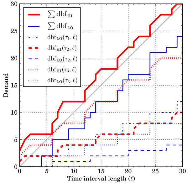
Fig. 5 Demand bound functions for the tasks from Example 1 with unmodified low-criticality relative deadlines ( D_i(\text{LO}) = D_i(\text{HI}) = D_i )
