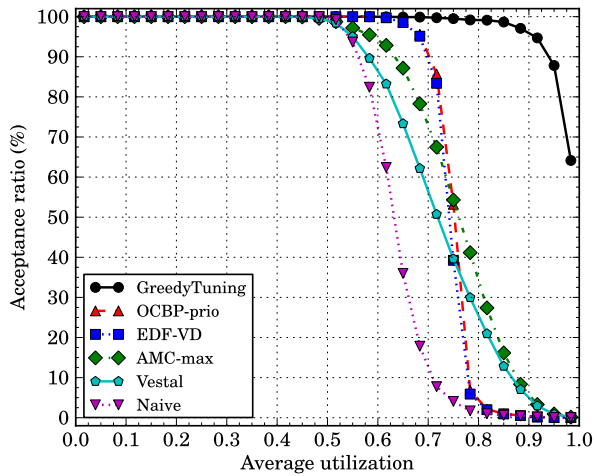
Fig. 10 P_{HI} = 0.5, R_C = 4, C_{LO}^{max} = 10, T^{max} = 200 and R_D = 1
