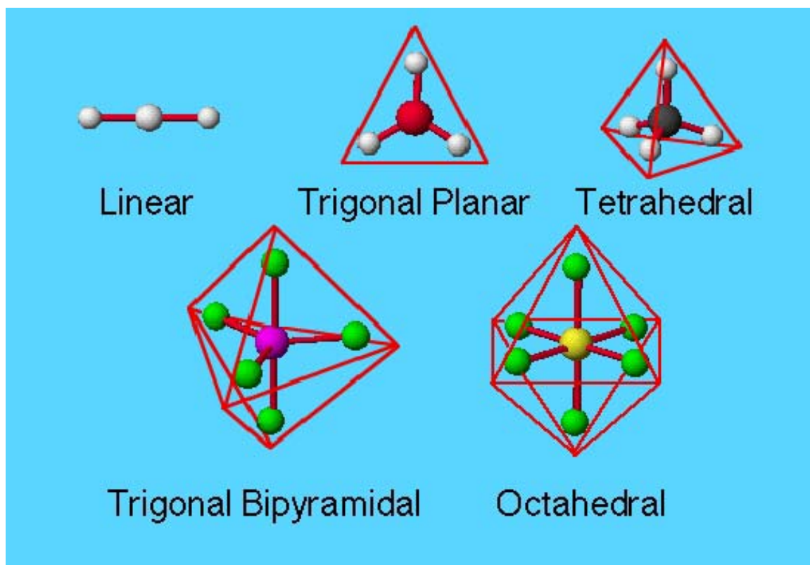
Figure 1. Molecular geometry types.
