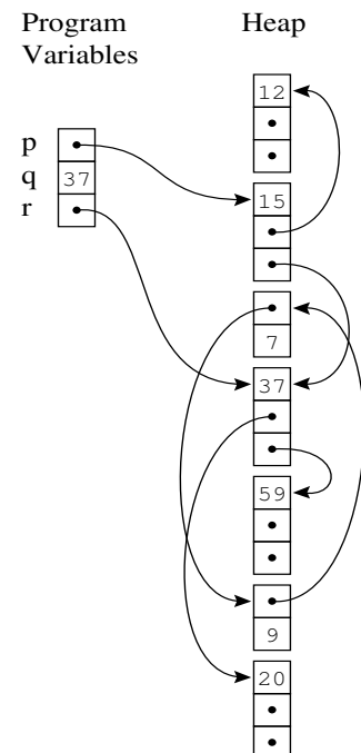
FIGURE 13.1. A heap to be garbage collected. From Modern Compiler Implementation in ML , Cambridge University Press, ©1998 Andrew W. Appel
