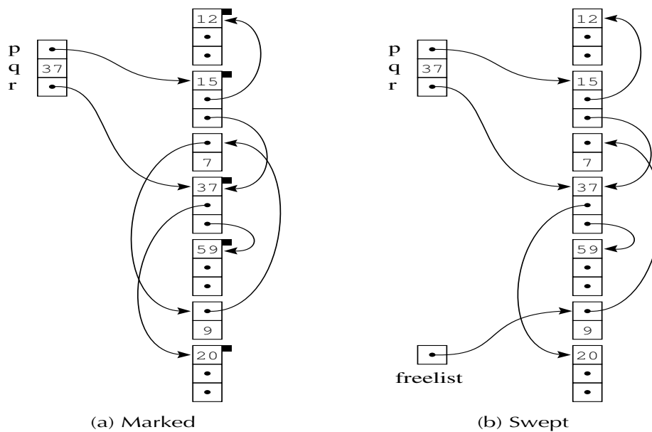
FIGURE 13.4. Mark-and-sweep collection. From Modern Compiler Implementation in ML , Cambridge University Press, ©1998 Andrew W. Appel
