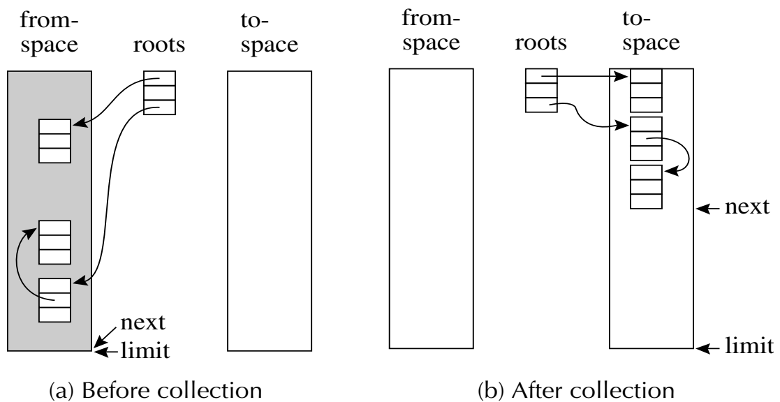
FIGURE 13.7. Copying collection. From Modern Compiler Implementation in ML , Cambridge University Press, ©1998 Andrew W. Appel
